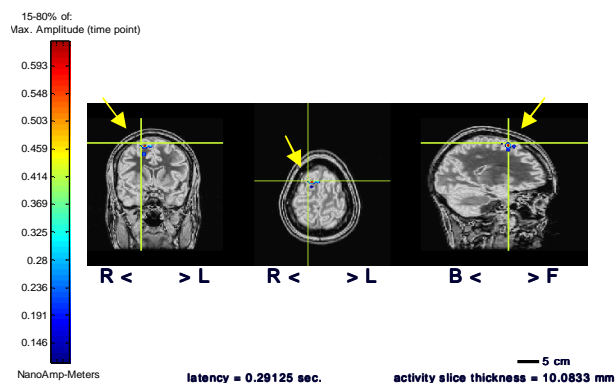
Fig. 2. Activation of Right Superior Frontal cortex in Female ADHD patient at 291 ms post-stimulus of CPT – Condition 2.
