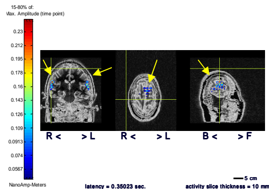
Fig. 3. Activation of Right and Left Inferior Frontal and Right Superior and Dorsolateral Frontal, and Right Parietal cortex in Male ADHD at 350 ms post-stimulus of CPT- Condition 3.
